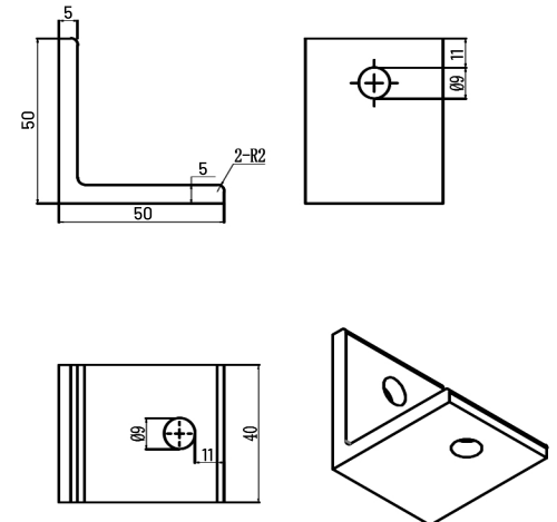
Alu-Winkel
